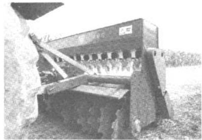
图6 2BMXD-12型小麦免耕播种机 Fig.6 2BMXD-12 wheat no-till seeder
