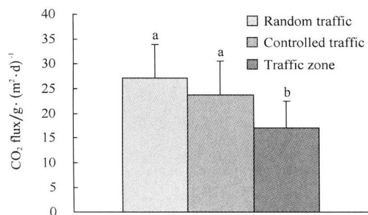
Figure 4 Soil respirations on inter row zone under random traffic and controlled traffic and traffic zone. Different lower case letter indicate significant ( P < 0.05 ) difference between inter row zone and traffic zone
